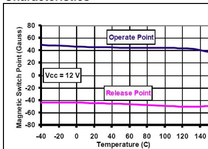
Figure 1. Typical Magnetic Characteristics
