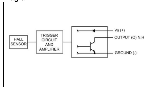
Figure 3. Current Sinking Output Block Diagram
