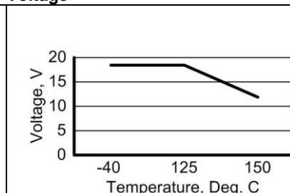
Figure 2. SS361RT Rated Supply Voltage
